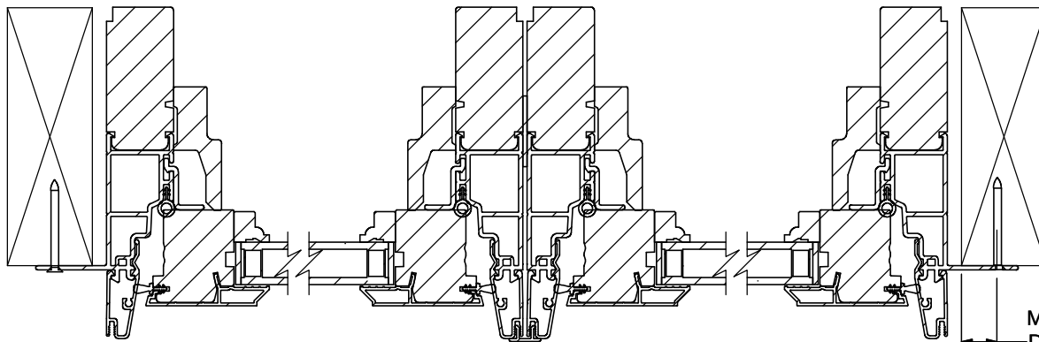
SECTION C-C SCALE 1 : 3
